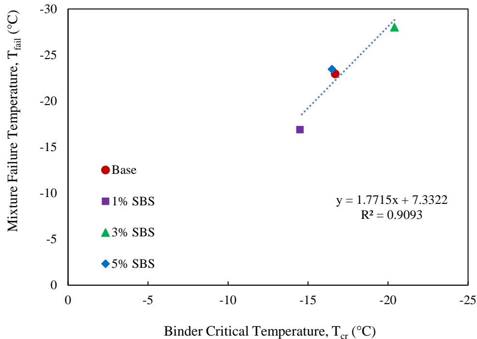
FIGURE 49 Binder critical temperature versus mixture failure temperature
