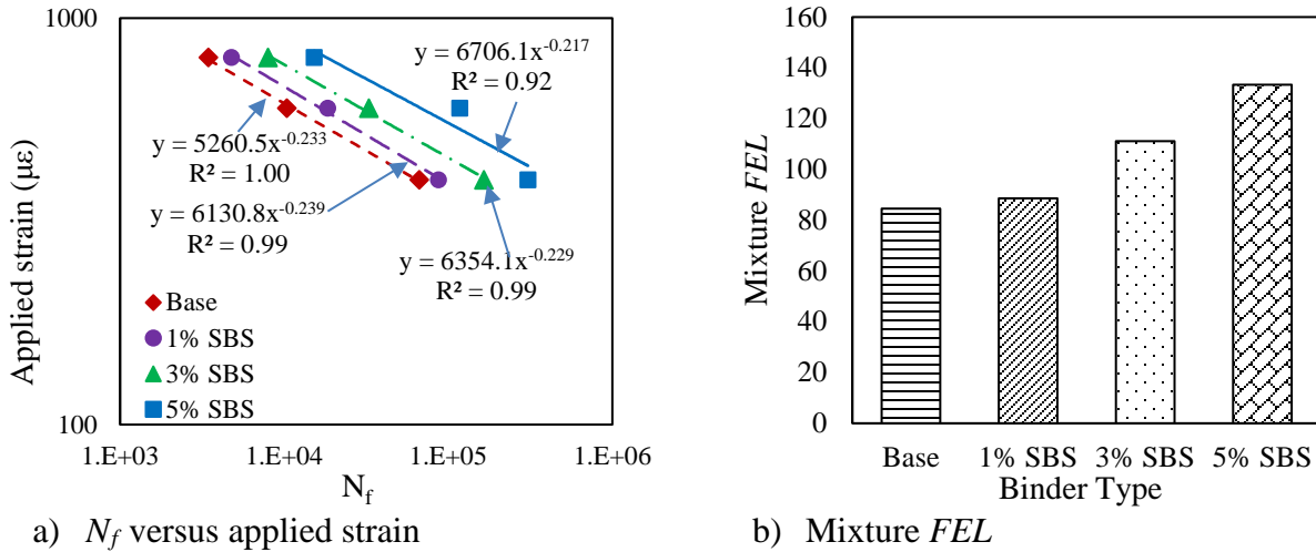
FIGURE 29 BF test results
