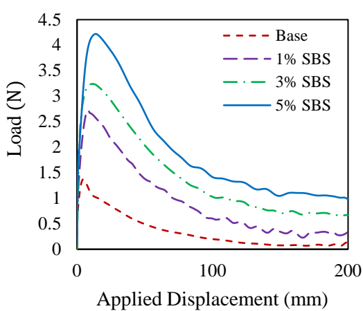
a) Load-displacement plot
