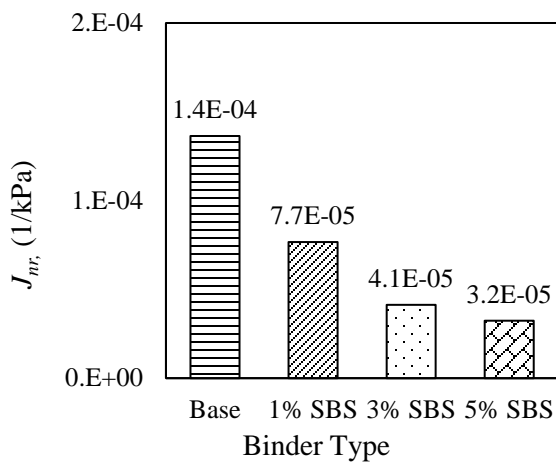
a) J_{nr} at 350 kPa
