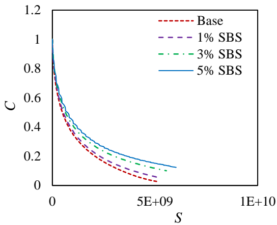
c) Damage curve
