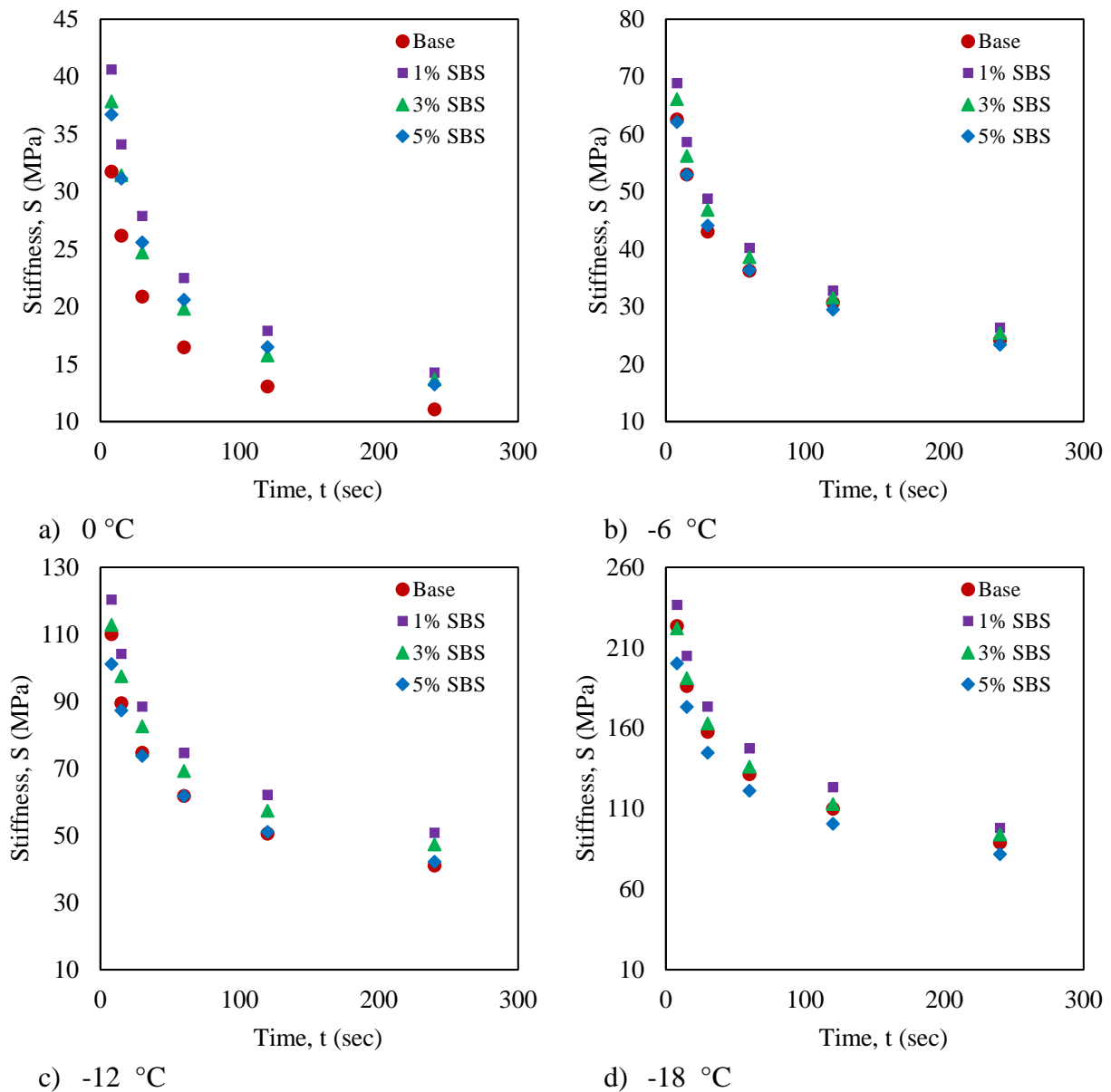
FIGURE 42 BBR Results
