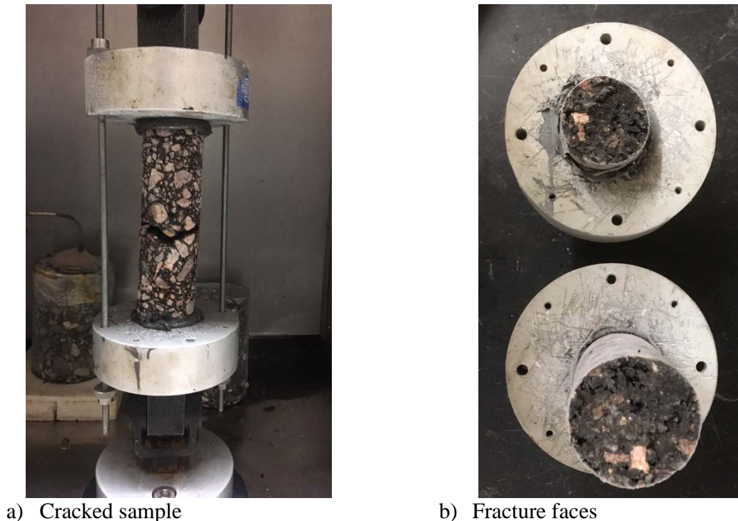
FIGURE 39 TSRST test
