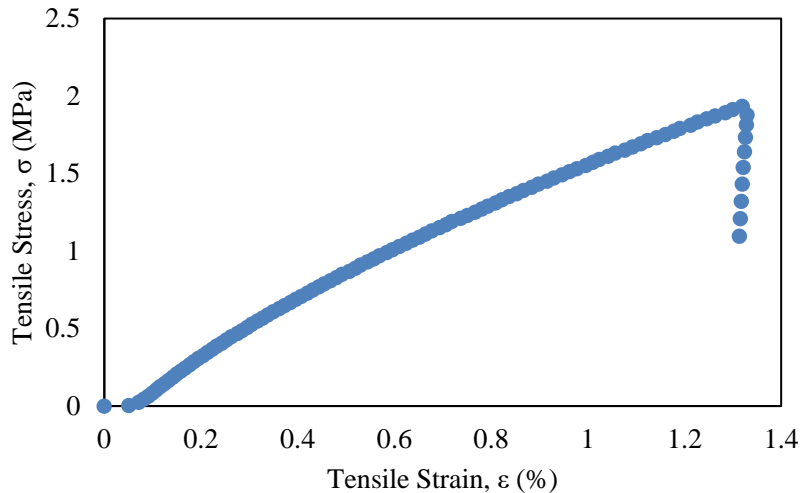
FIGURE 47 DT test result for 3% SBS at -24\text{ }^{\circ}\text{C}
