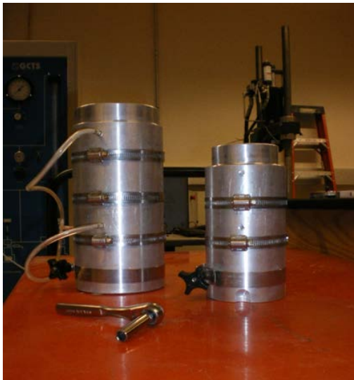
2.8" and 4" diameter subgrade soil mold 6" diameter base soil mold with compacted soil
