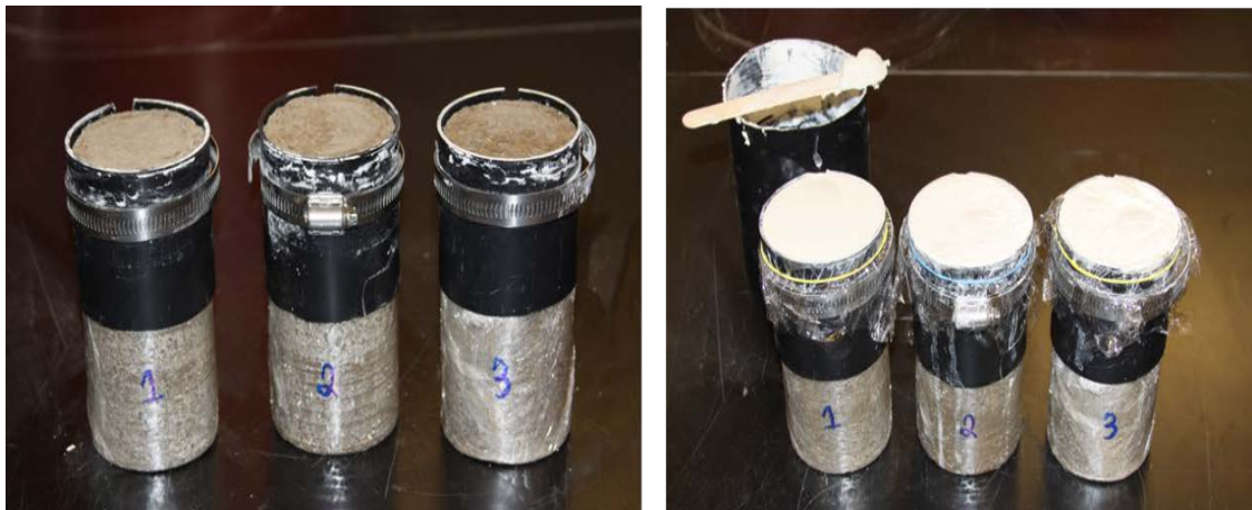
Figure 4.4: Capped Plastic Wrap Subgrade Samples
