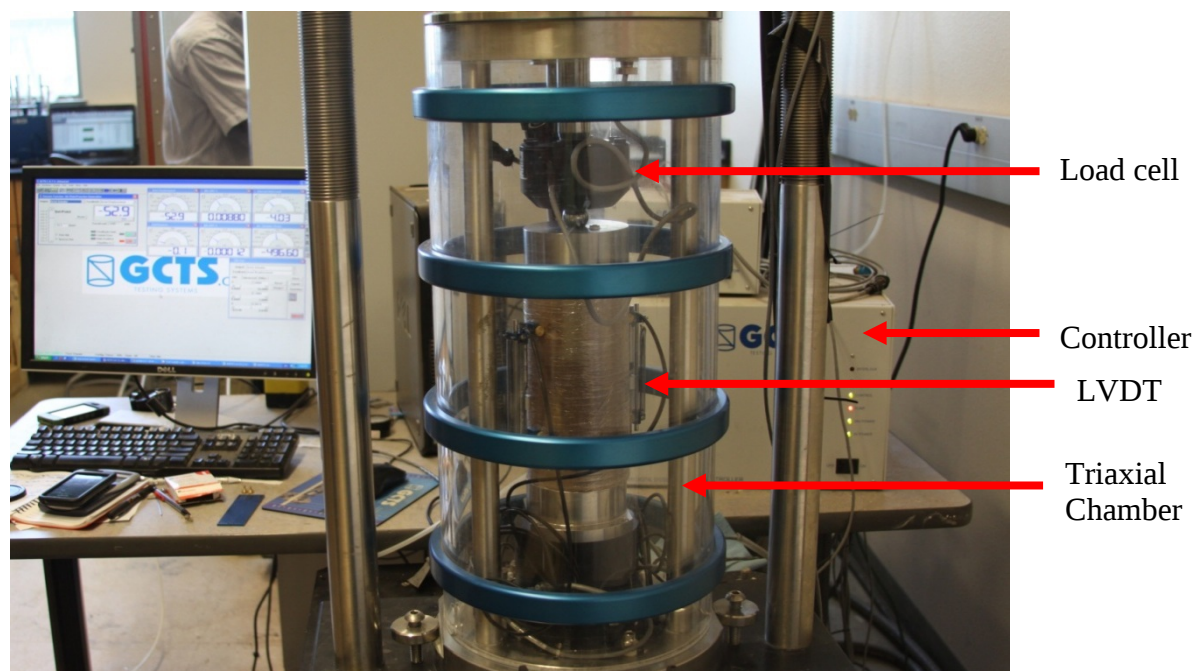
Figure 4.9: Subgrade Resilient Modulus Test Setup in Triaxial Chamber
