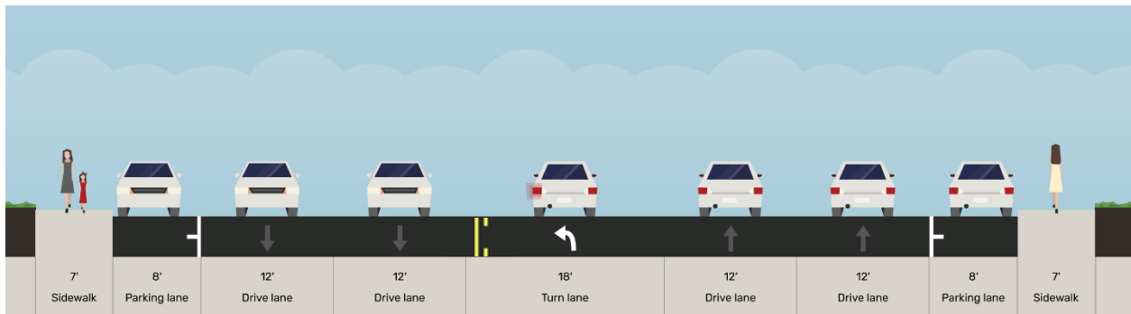
FIGURE 19. Cross section diagram of US-60 / California Street in Socorro, NM (note that the center left-turn lane alternates which side of the street it serves)
