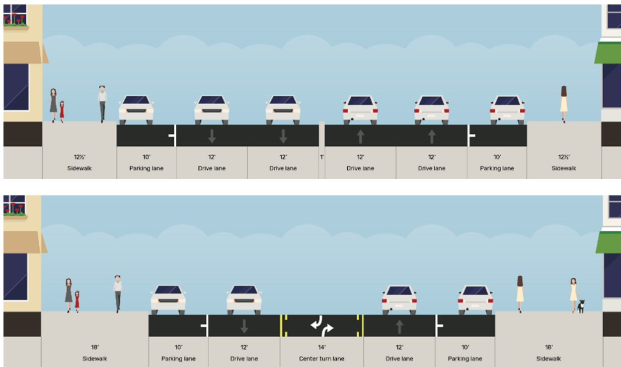
FIGURE 29. Cross section diagram of Highway 78 / Lake Avenue in Battle Lake, MN before (top) and after (bottom) road redesign
