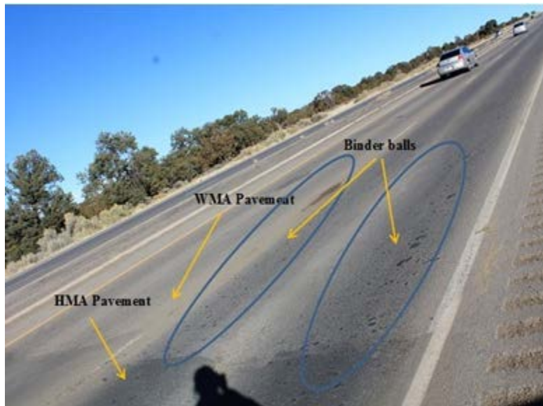
FIGURE 19 Binder Balls.
