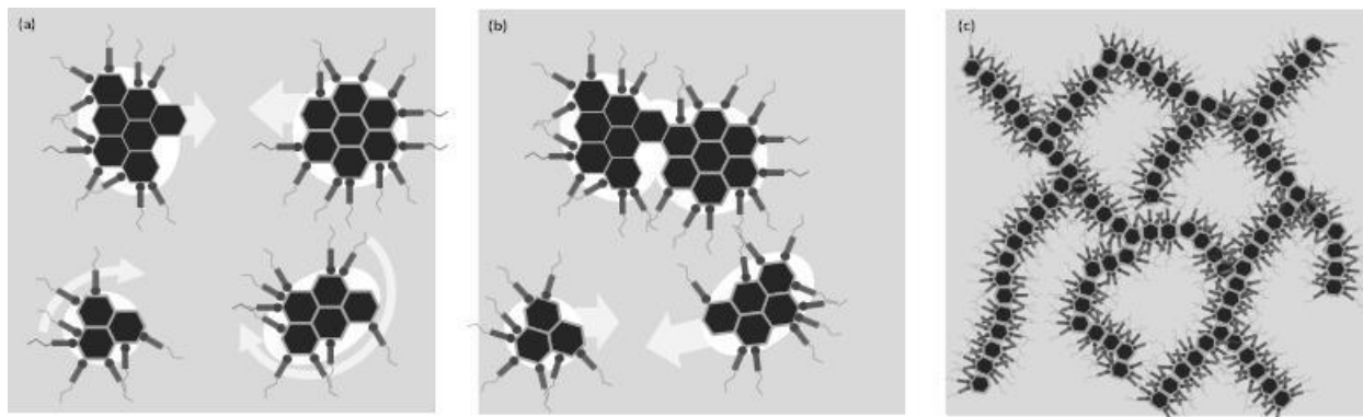
Figure 7. When the ratio of resins to asphaltenes decreases, attraction between partially peptized asphaltene surfaces (a) lead to the formation of structures that resist shear (b,c). Binders that exhibit this type of behavior are known as GEL binders.
