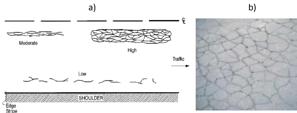
Figure 11. Fatigue cracking: (a) severity of fatigue cracking, and (b) fatigue cracking image (41).
